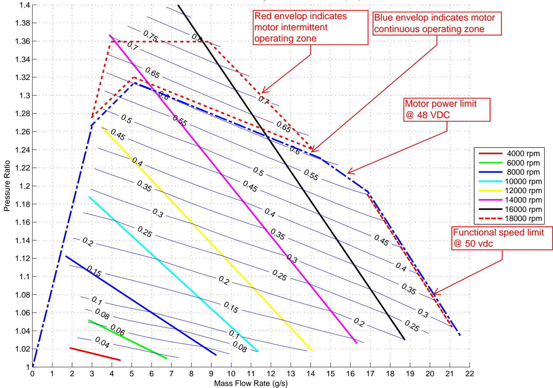
VRB10-X102 Massflow vs Pressure Ratio with System Power Contours (kW) at Sea Level
