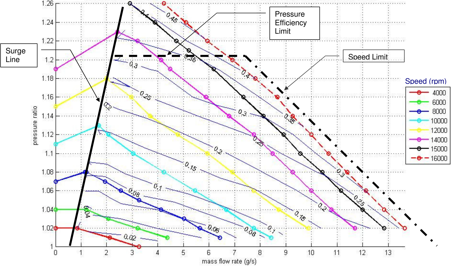
Characteristic VR612 090807 Massflow vs Pressure Ratio with System Power Contours (kW) at Sea Level
