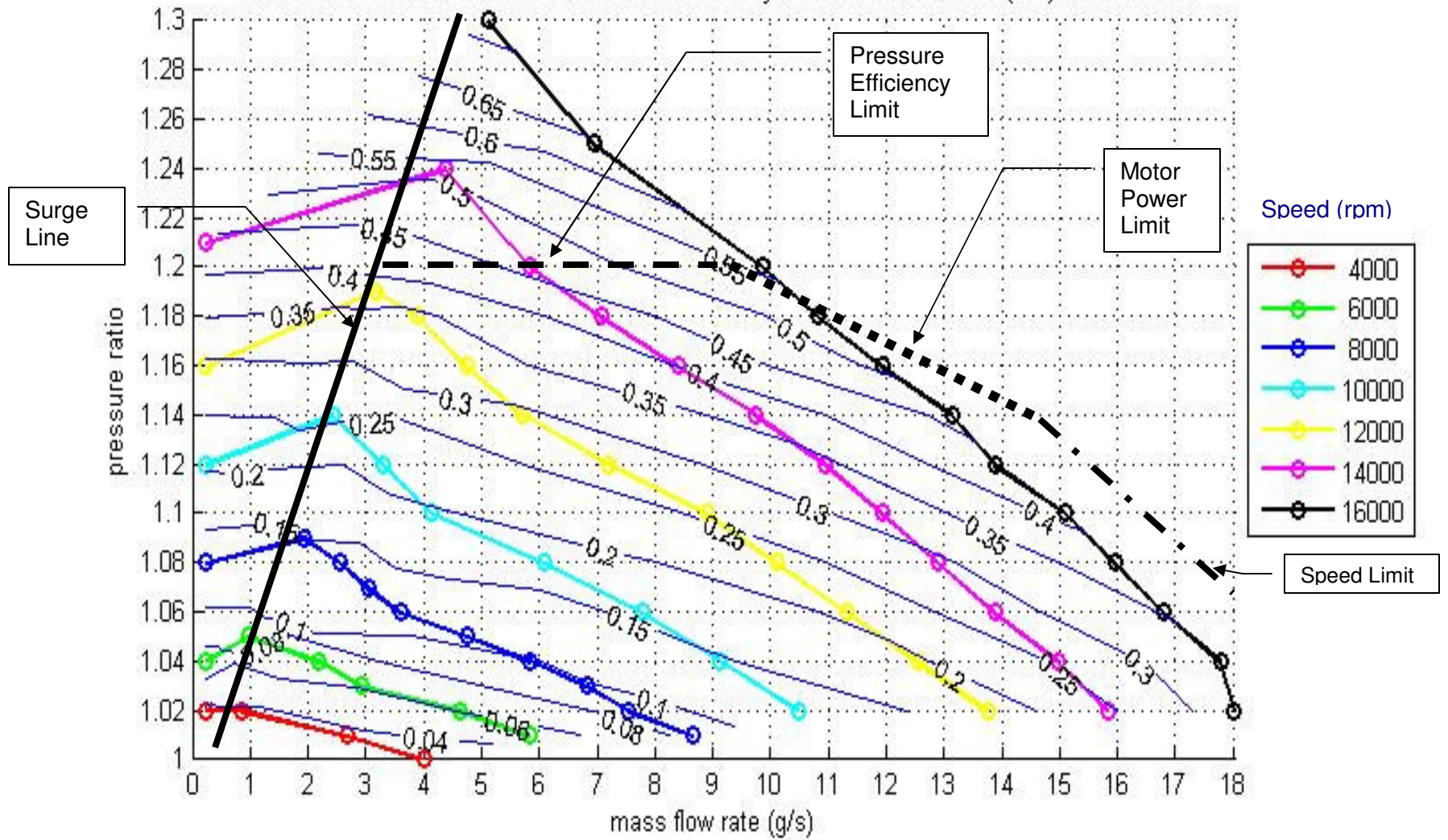
VR1012.01 48V Massflow vs Pressure Ratio with System Power Contours (kW) at Sea Level
